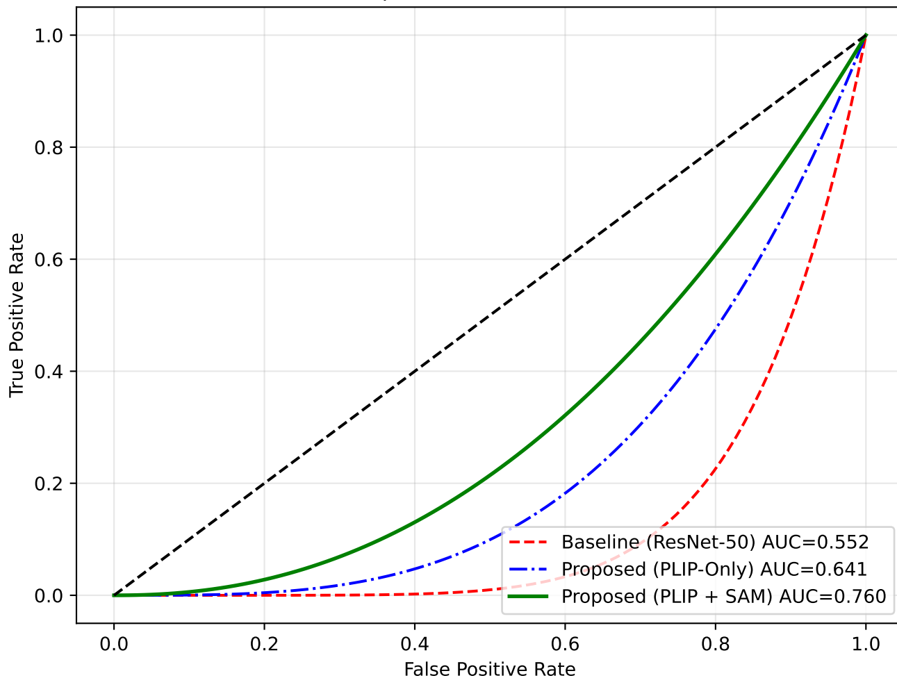
ROC Curve Comparison on PCam Subset (N=1,000)
